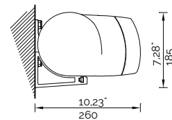
Wall installation
