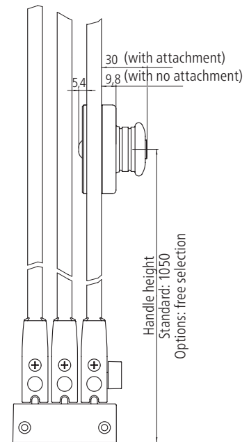
Cup pull handle, both options
