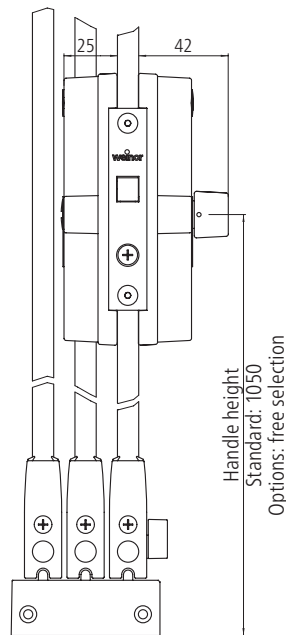
Knob for lockcase and hung bolt
