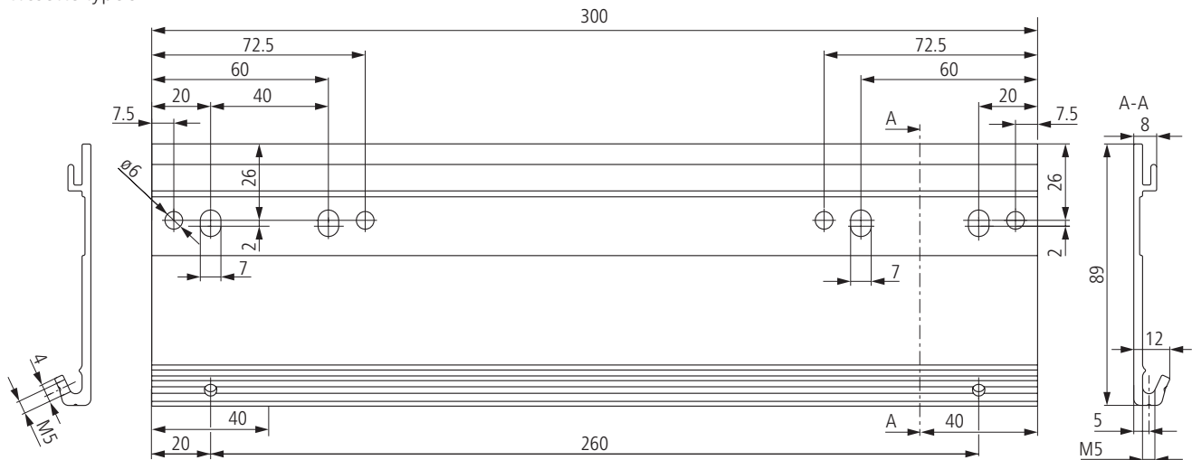
cassette type 92/112
