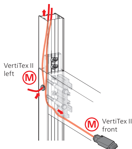
Hirschmann plug is pre-assembled at the factory
