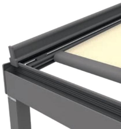
Headplate bracket
