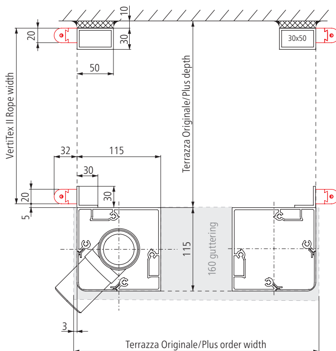
VertiTex II Rope lateral
