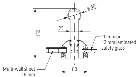
L roof support
