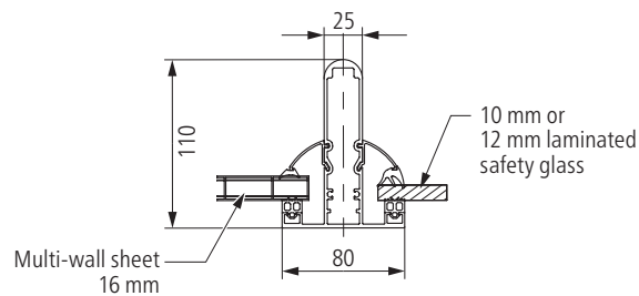
S roof support
