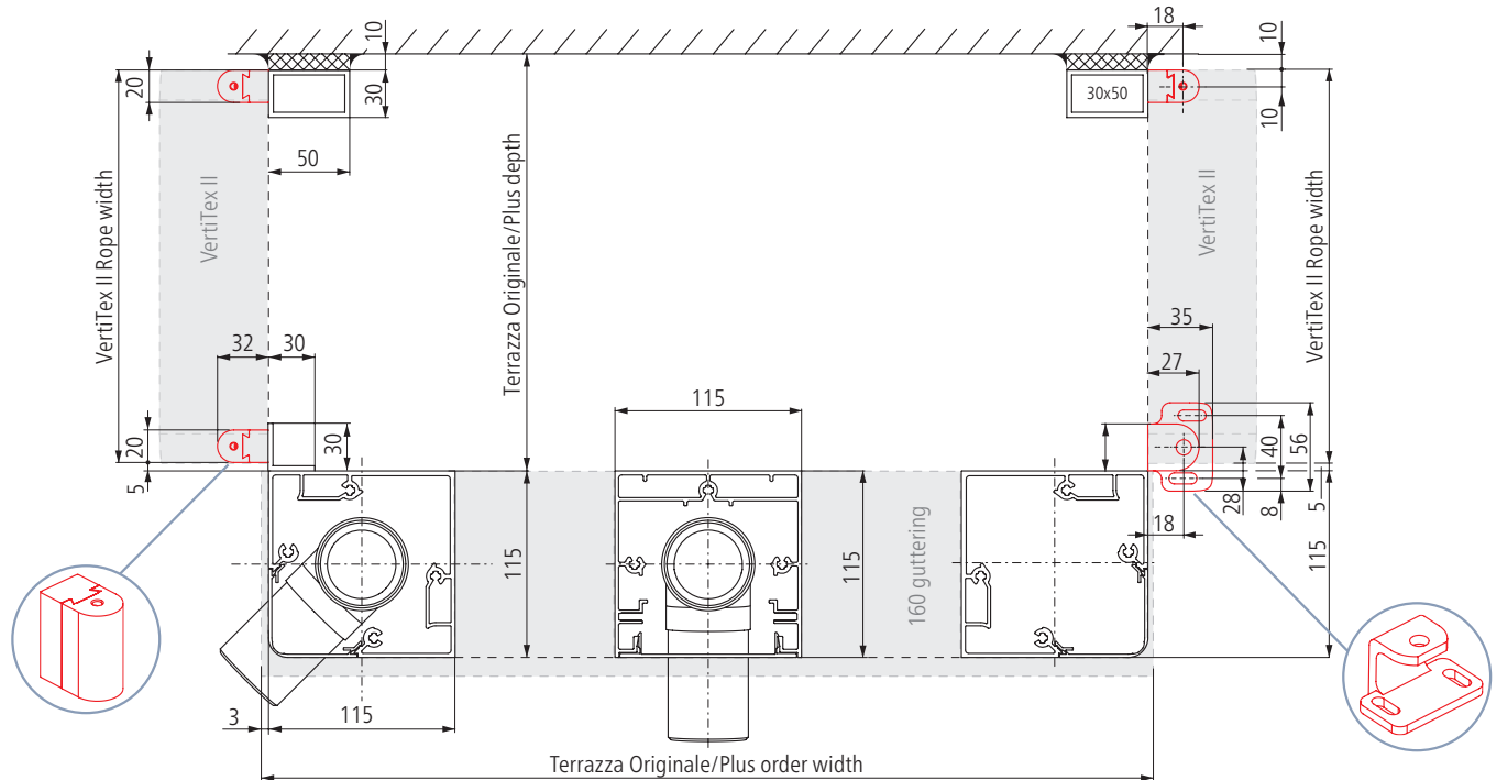
VertiTex II Rope lateral
