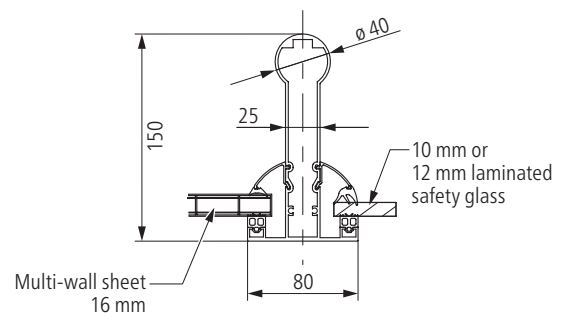
L roof support
