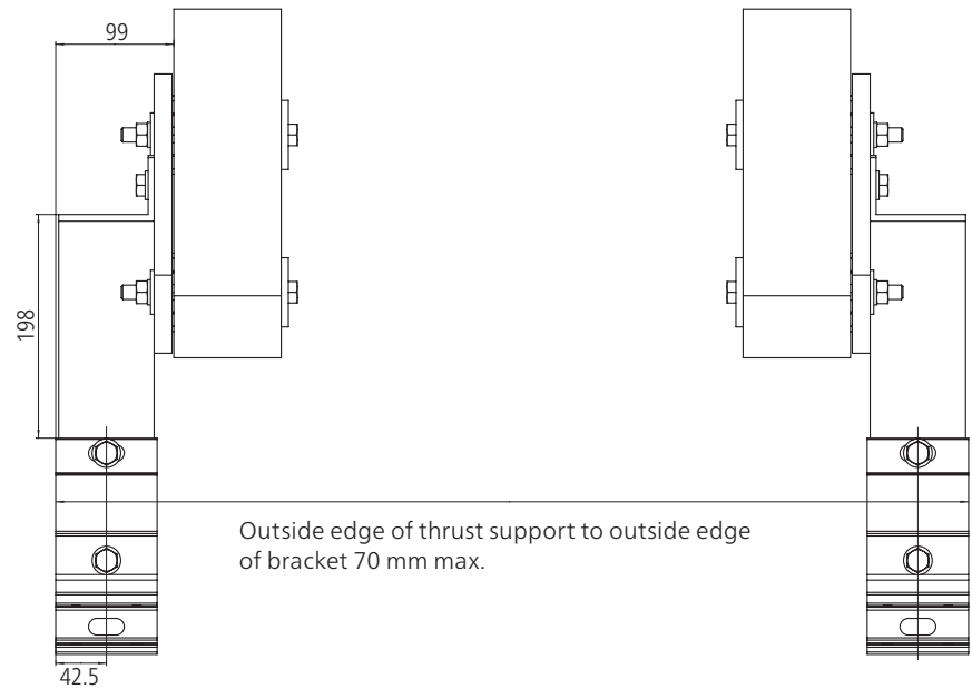
Rafter mounting
