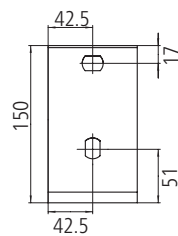
Ceiling bracket
