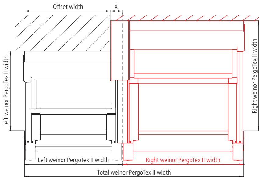
Multi-section unit with offset (top view)
