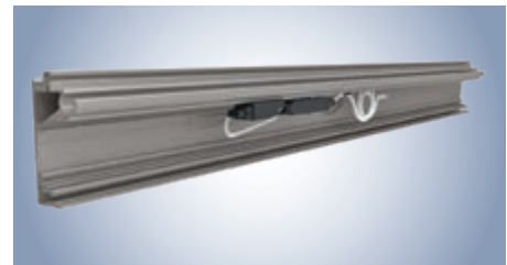
Wall connection profile with BiRec MA-K (without LED option)
