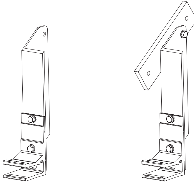
Rafter bracket with mounting plate for right-hand rafter weinor recommends using mounting plates for rafter brackets
