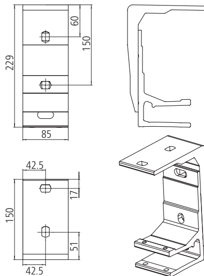
Ceiling bracket
