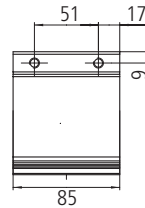
85 mm wall bracket
