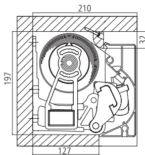
Type N niche installation
