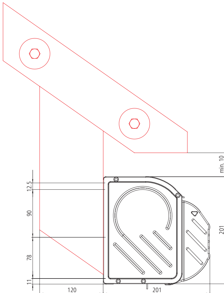
Rafter bracket with mounting plate for right-hand rafter weinor recommends using mounting plates for rafter brackets
