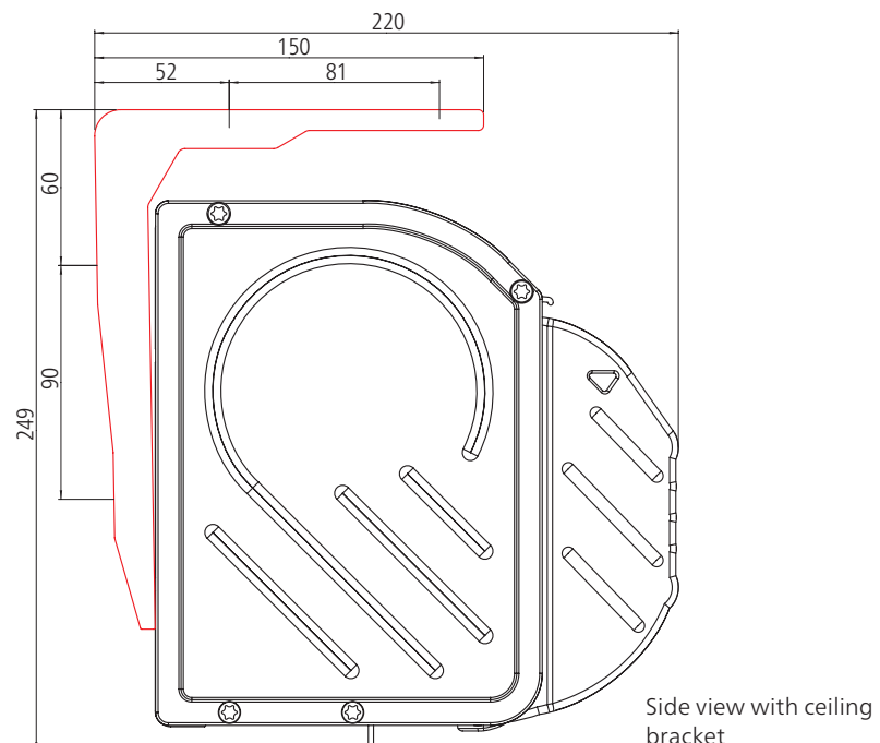
Ceiling bracket
