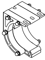
top fixture bracket 135 mm 5°–35°
