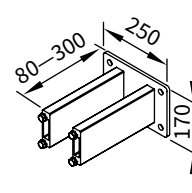
stand-off bracket for face-fixture bracket 77921. and 77936.
