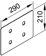
cover plate for spacer plate and stand-off brackets in the case of external insulation
