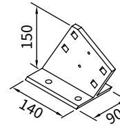
eaves fixture bracket 150 mm
