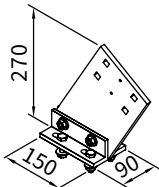
eaves fixture bracket 270 mm please refer to "Eaves fixture with spreader / backing plate"
