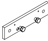
supplementary flat plate eaves fixture 260 × 60 × 12 mm please refer to "Eaves fixture with spreader / backing plate"
