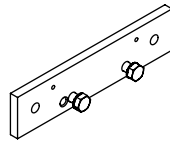
supplementary flat plate eaves fixture 260 × 60 × 12 mm please refer to "Eaves fixture with spreader / backing plate"
