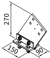
eaves fixture bracket 270 mm plate please refer to "Eaves fixture with spreader / backing plate"
