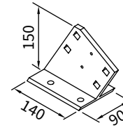
eaves fixture bracket flat plate 150 mm
