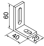
angled bracket 60 × 40 × 25 mm please order additional accessories 799141!
