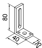
angled bracket 80 × 40 × 25 mm please order additional accessories 799141!
