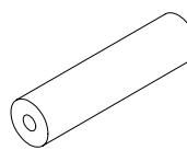
stand-off fixing tube 30 × 10 × 1000 mm N.B! max. stand-off distance 120 mm
