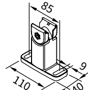
track bracket with adjust- able head fixture type 21 100 mm
