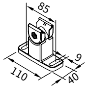
track bracket with adjustable head fixture type 20 80 mm
