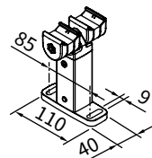
double track bracket with adjustable head 140 mm
