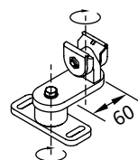
universal track bracket 80 mm
