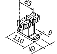
double track bracket with adjustable head central bracket for 2 single units next to each other 80 mm
