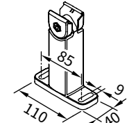
track bracket with adjustable head fixture type 22 140 mm
