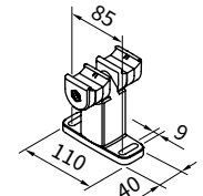
double track bracket with adjustable head central bracket for 2 single units next to one another 100 mm
