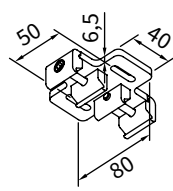
double track bracket flat 2 single units
