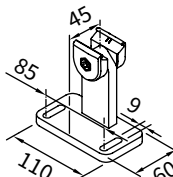
track bracket with adjust- able foot plate 100 mm
