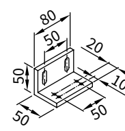
additional angled bracket for the bearing, gearbox and motor sides fixture type 15 50 × 50 × 80 mm
