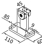
track bracket with adapter plate
