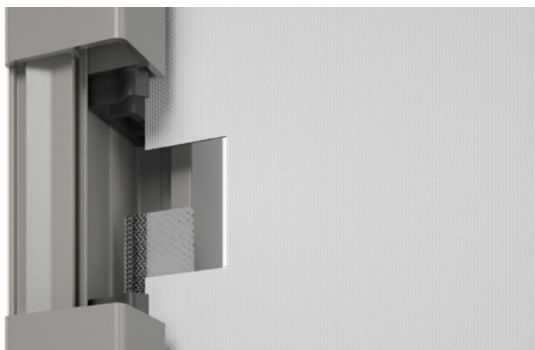
section of guide rail with tracfix profile
