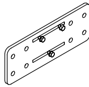
spreader plate A face fixture 160 × 430 × 12 mm
