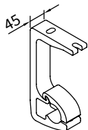
top fixture bracket
