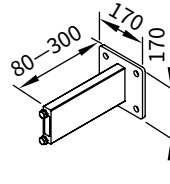
guide rod bracket for face fixture bracket 71813.
