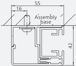
Wall mounting
