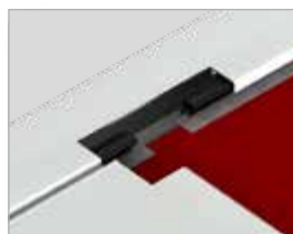
cut-out section of guide track with zip system and internal plastic zip profile
