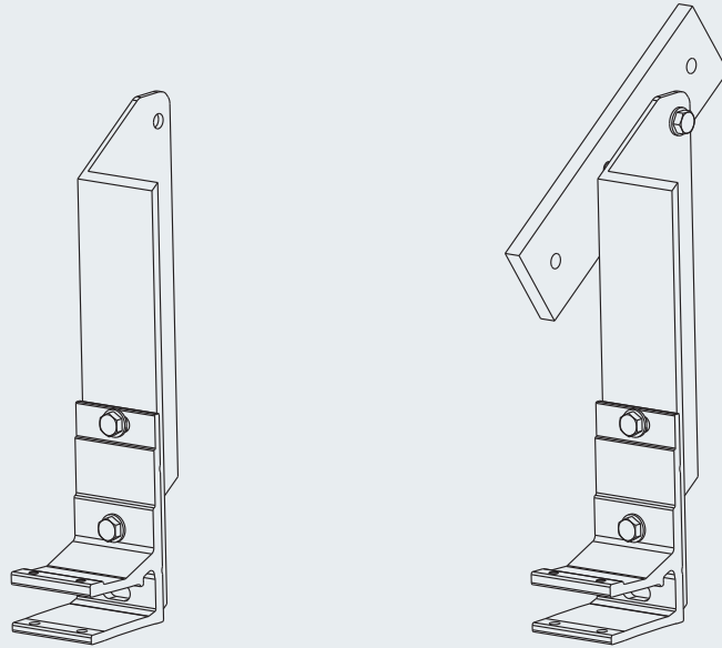
Rafter bracket with mounting plate for right-hand rafter weinor recommends using the mounting-plate for rafter brackets.
