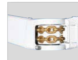
to protect them from corrosion the strong double steel-link chains are recessed into the elbow joints of the folding arms
