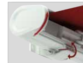
pitch adjustment via the fixture brackets
